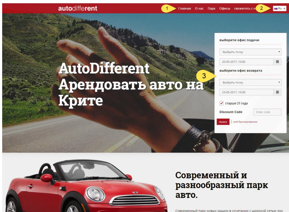
Screenshot 1
