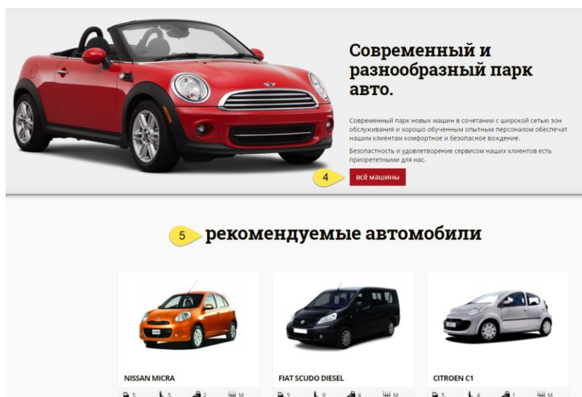
Screenshot 2
