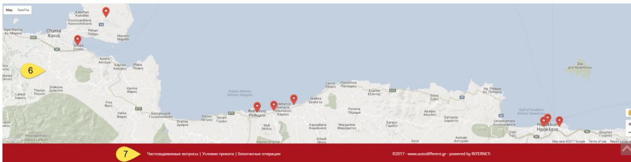
Screenshot 3
